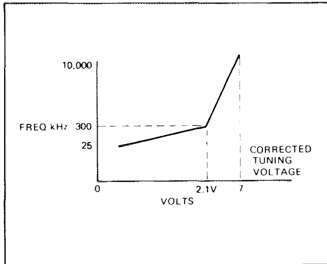
Figure 9E-4-3. VCO Characteristics
