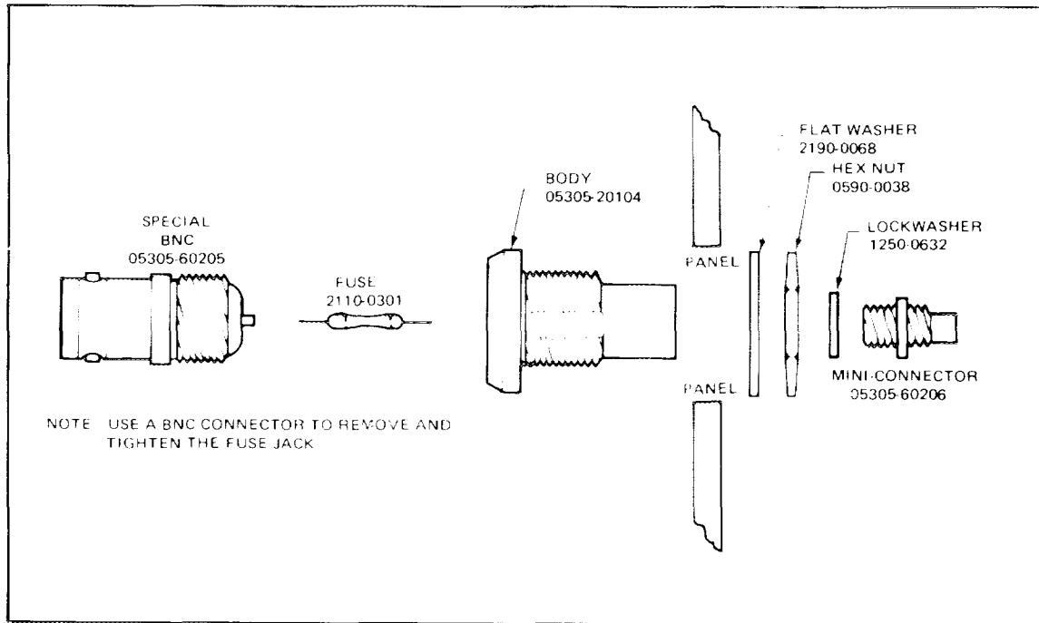
Figure 6-1. Details of Input Connector J1 and Fuse Mounting
