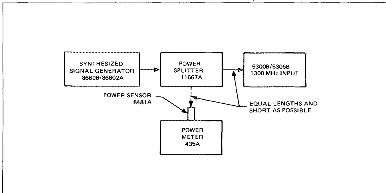
Figure 9E-5-2. Test Setup for 1300 MHz Adjustment
