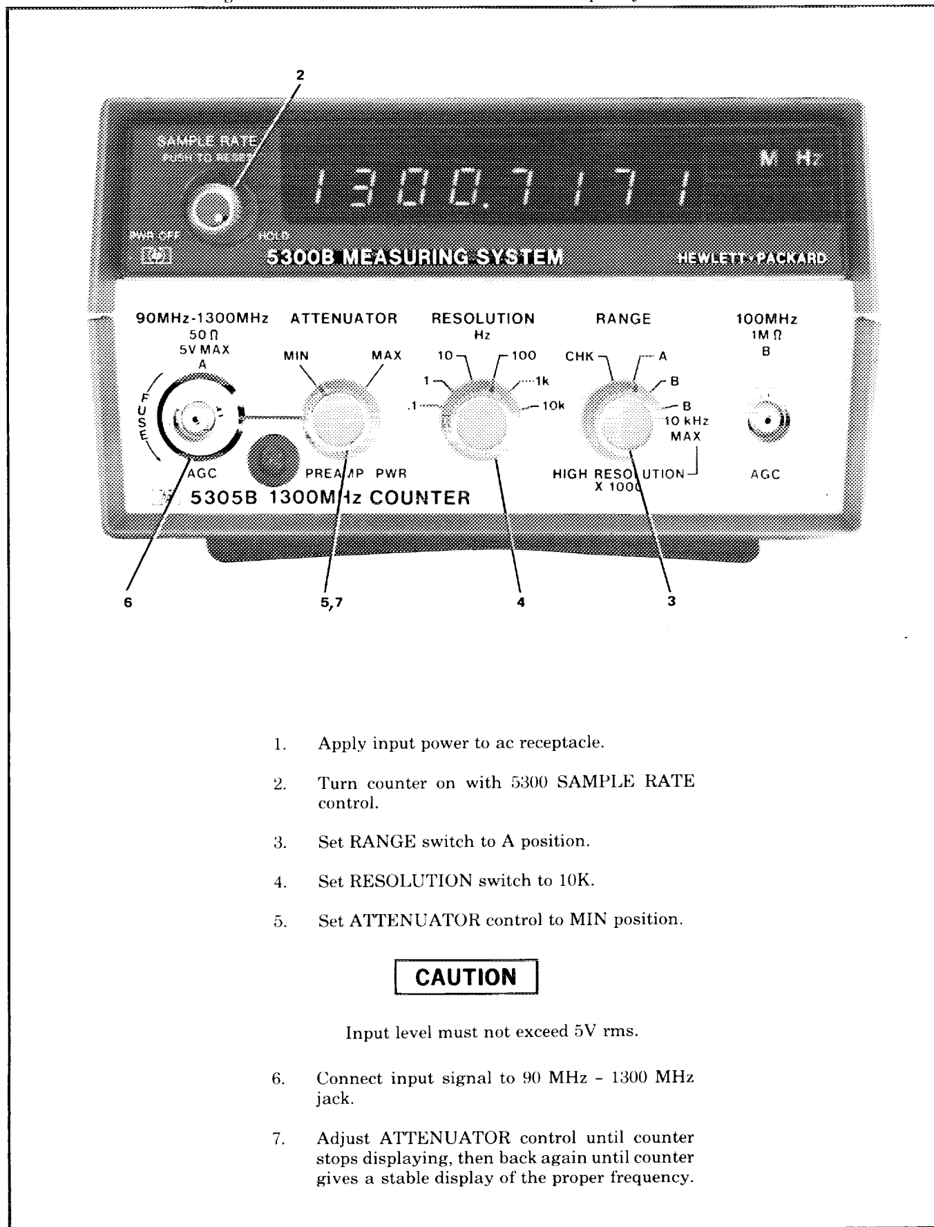
Figure 9E-3-5. 90 MHz - 1300 MHz Channel Frequency Measurements
